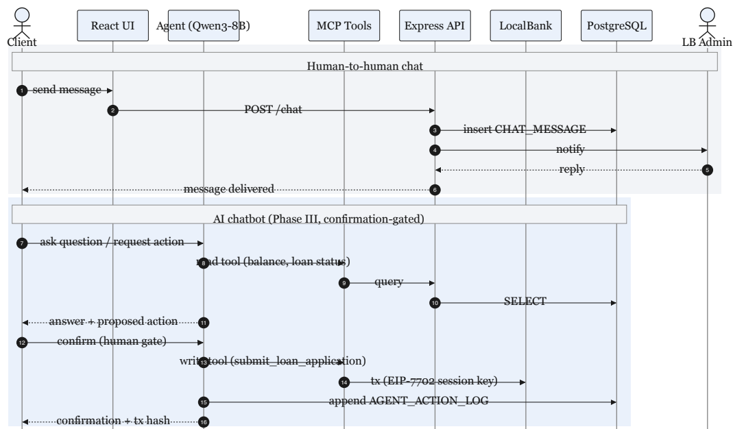
Figure 3.31: Sequence diagrams
