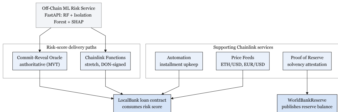
Figure 3.4: Oracle architecture
