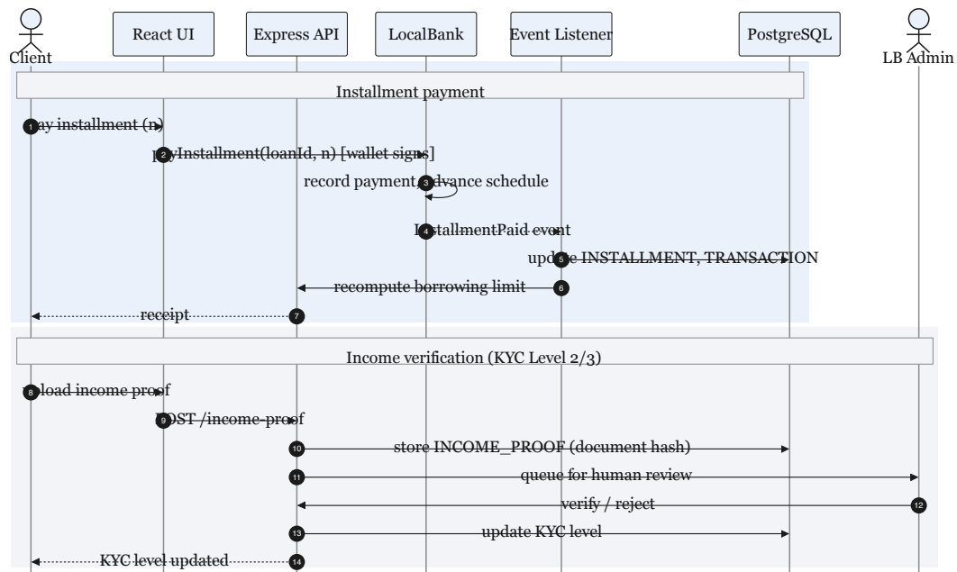
Figure 3.29: Sequence diagrams
